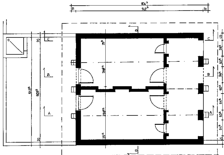
Fig. 286: Guest house: plan of masonry walls 29.5 and 14 cm thick.
