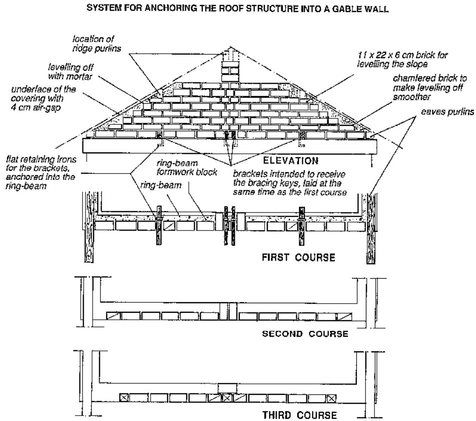
Fig. 224: Elevation and coursing of the block courses at the top of the gable wall to include a system of anchoring of the roof structure using braced brackets.
