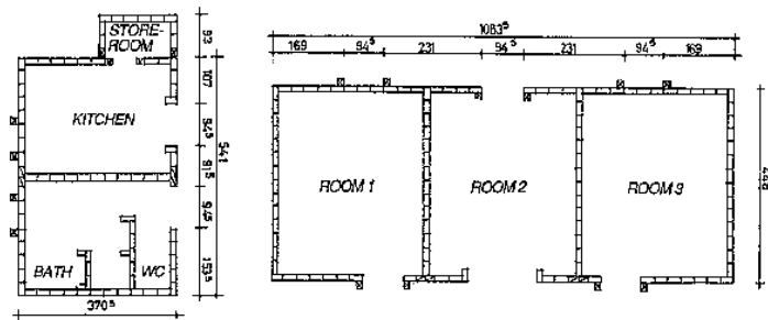
Fig. 212: Plan with coursing of the first layer of blocks of the basic T3 type.
