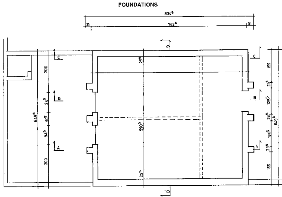
Fig. 287: Guest house: plan of Cyclopean concrete foundations.
