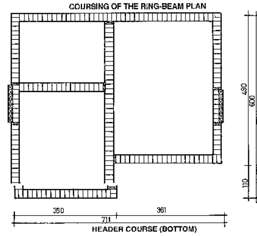
Fig. 266: Course of header blocks forming the bottom of the formwork for the ring-beam.
