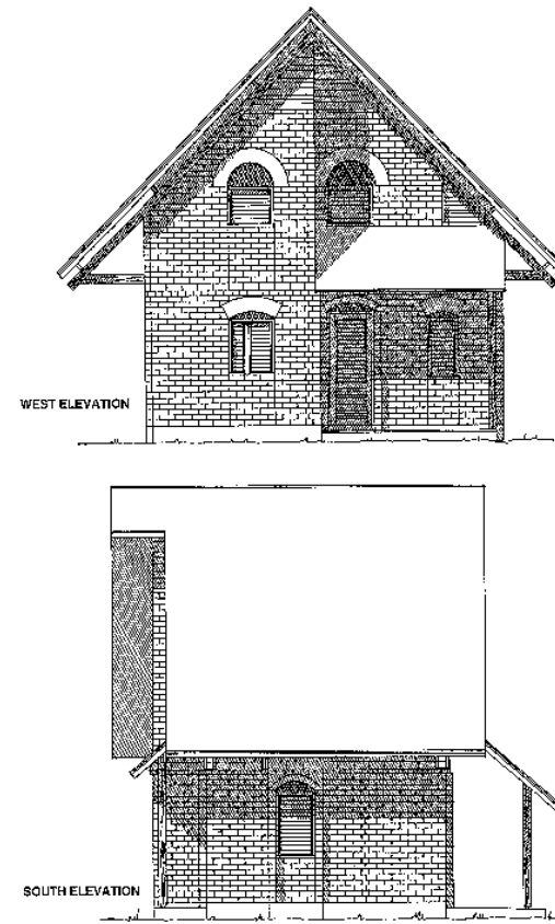
Fig. 262: West and south elevations: access to the main elevation is by a small stepped verandah.
