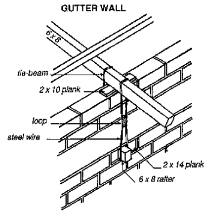
Fig. 142: Detail of anchoring the rafter at the lower end using a system of stainless steel tie rod and stainless steel wire tension strap.
