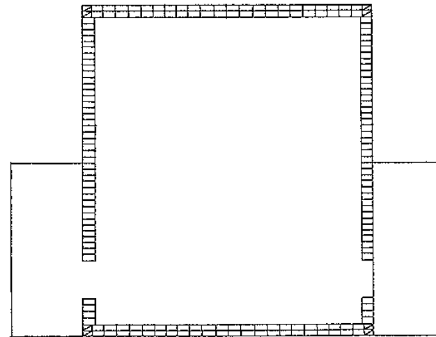
Fig. 304: Coursing of bonding pattern of the first four odd number courses 29.5 cm thick (footing).
