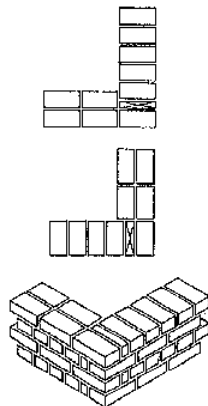
Fig. 58 a: Corner bonded using headers and stretchers without three-quarter blocks.
