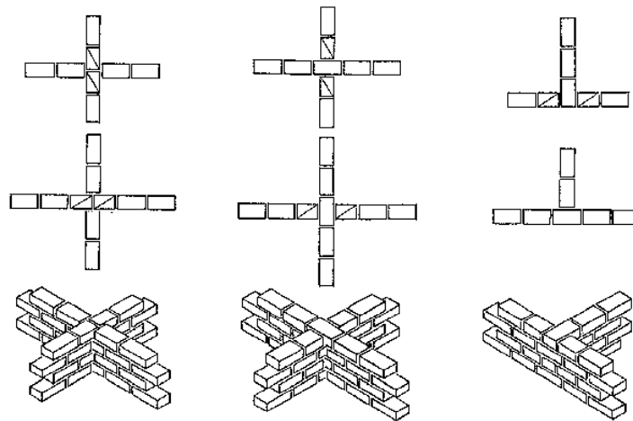
Fig. 52: "T"-shaped bonding pattern using three-quarter blocks
