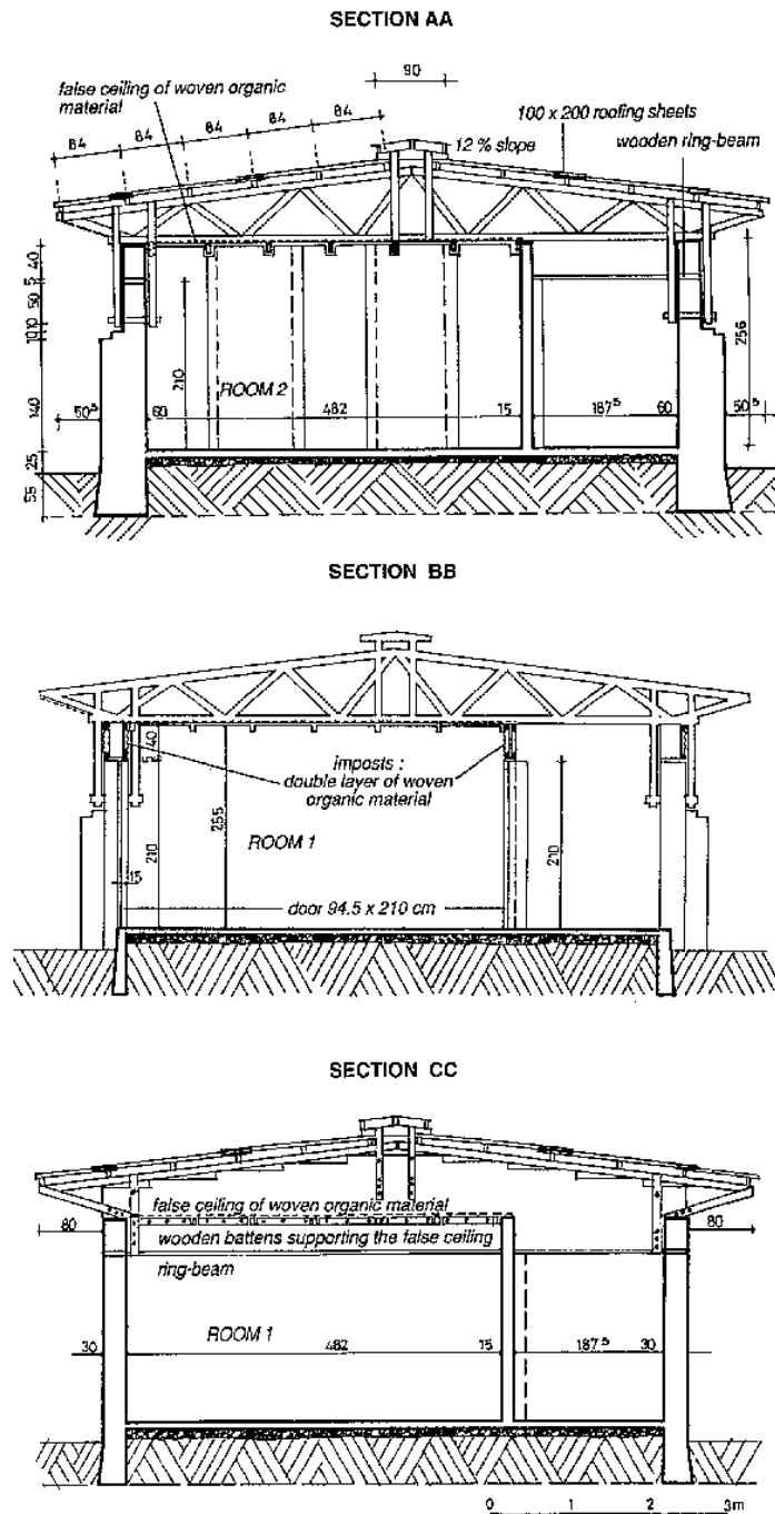
Fig. 289: Three transverse sections of the guest house, at different levels (see plan). Note the false ceiling of woven organic material.
