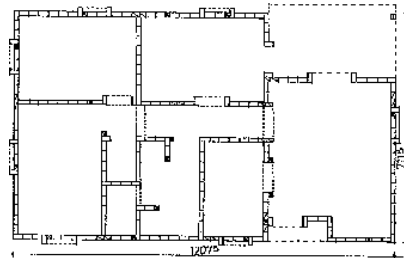
COURSING OF THE FIRST COURSE OF BLOCKS
