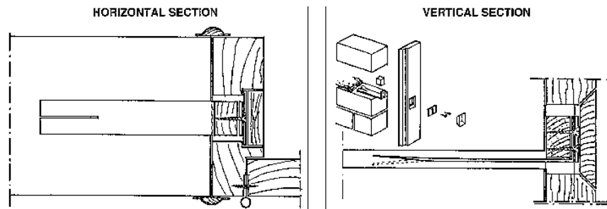
Fig. 279: Detail of system of attachment using metal elements in the mortar.
