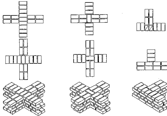
Fig. 56: "X" -shaped and bonding patterns using full blocks and "T"-shaped bonding patterns using three-quarter blocks.
