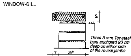
Fig. 246: Detail of moulded reinforced concrete window-sill and reinforcement of the receiving bed.
