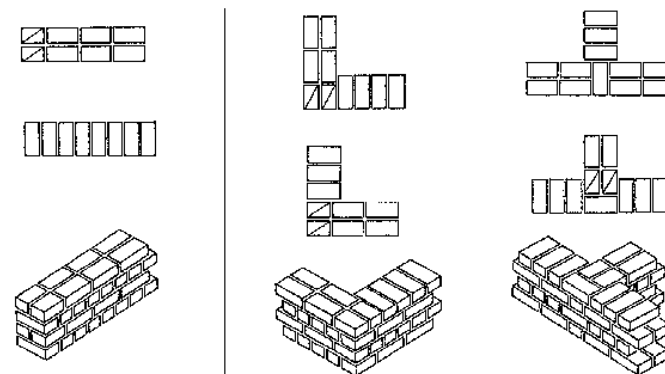
Fig. 54: Three-quarter block alternate courses and continuous wall.
