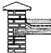
Fig. 146: Detail of water-proofing between roof/ parapet and roof/wall. Note the flexible system of laying of beams into the wall with insulation (thermal bridge) and waterproofing of the receiving base.
