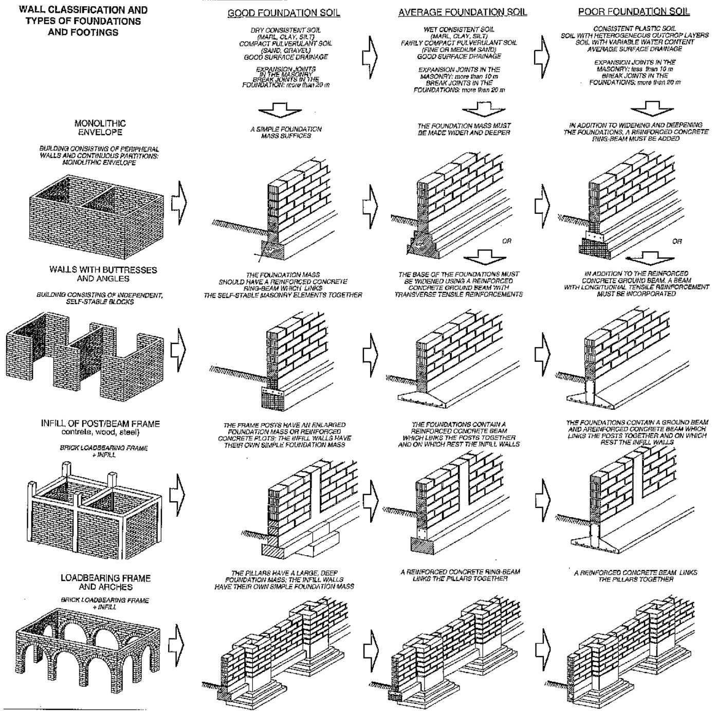
Fig. 81: Summary table of structural concepts depending on the type of wall and the nature of the ground for the foundation.
