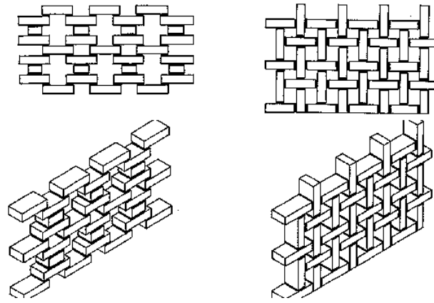
Fig. 158: Simple claustra-work designs with criss-cross motifs (full and half blocks) or the woven effect of stretchers with vertical blocks.
