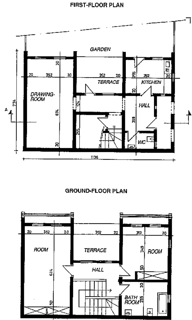
Fig. 234: Plan of house built in vibration-compacted blocks measuring 40 x 20 x 20 cm.
