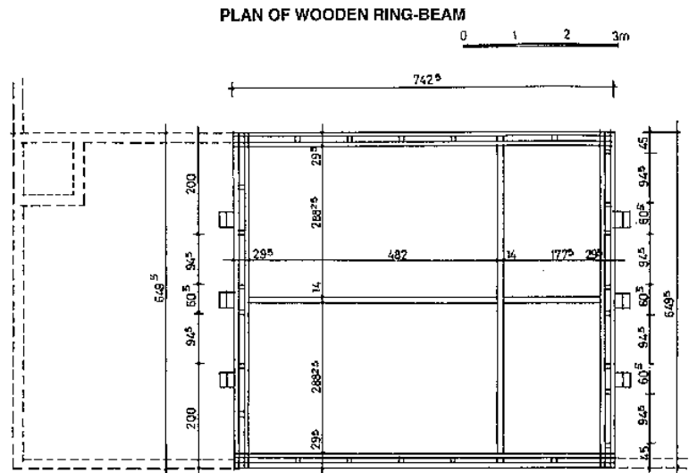
Fig. 296: Plan of laying of wooden ring-beam around the top of the 29.5 cm thick walls.
