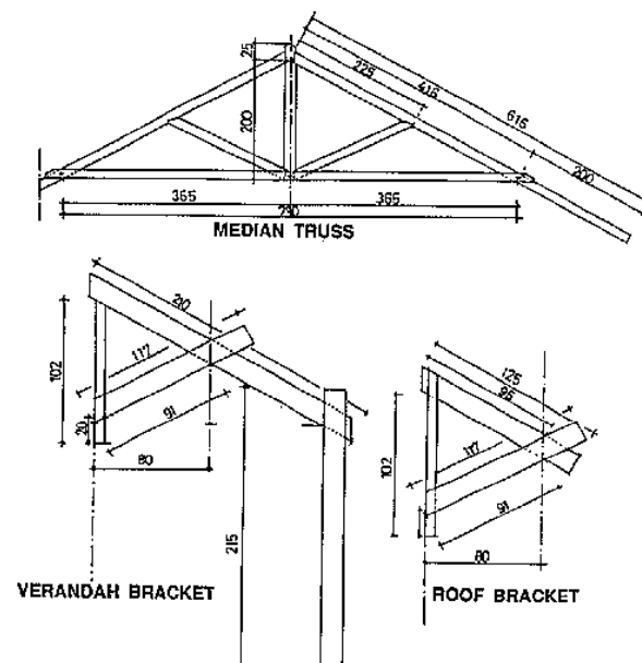
Fig. 313: Elevation of roof structure and details of roof and verandah brackets.
