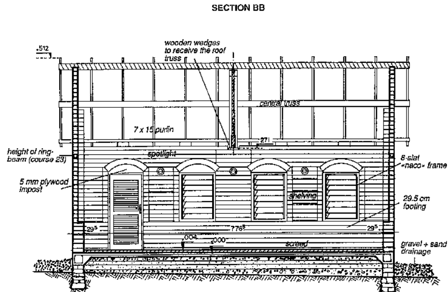
Fig. 311: Longitudinal section of classroom. Note
