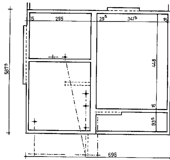
Fig. 263: Plans of foundations. Above, blinding concrete poured into gullies on which rests a reinforced concrete ground beam (lower plan).
