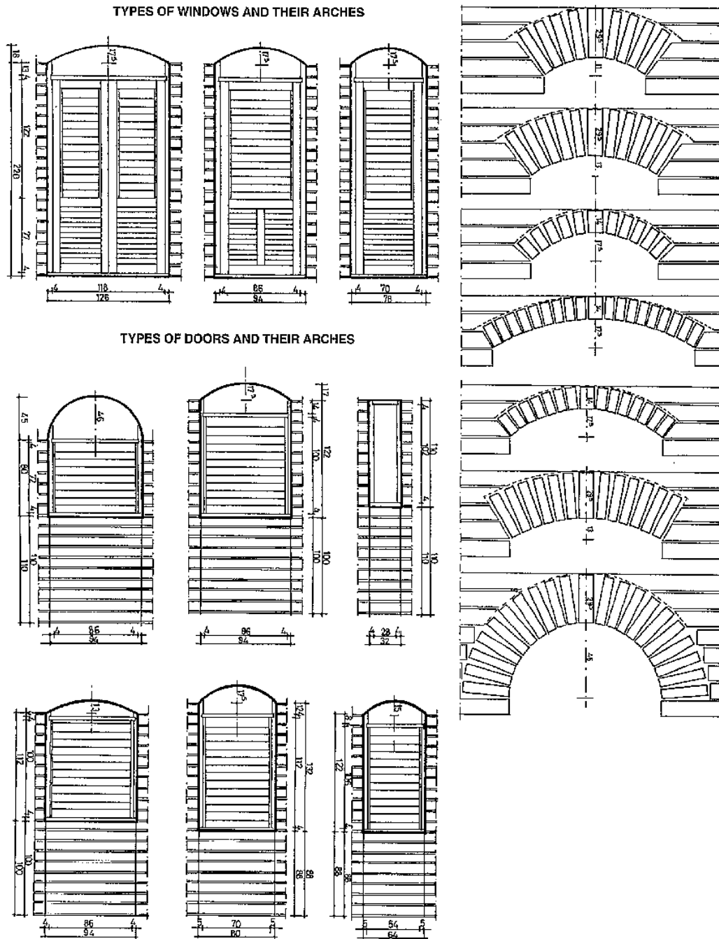
Fig. 277: Drawings of the complete range of door and window openings with Dutch or semi-circular arches.
