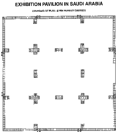
Fig. 324: Coursing of wall bonding patterns and arch and cupola pillars, for even number courses.
