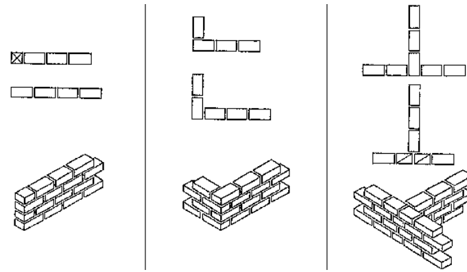
Fig. 50: half block used at the end of alternate courses and continuous wall.
