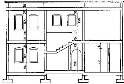
Fig. 237: Elevation and section M of house made from vibration-compacted blocks measuring 40 x 20 x 20 cm.
