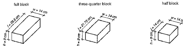
Fig. 48: Terms and rules for block dimensions using simple bonding patterns.
