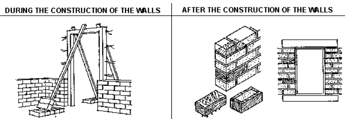
Fig. 106: Holding the door-frame in place as the walls are built up.
