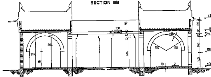
Fig. 320: Elevation of pavilion elevations and sections of exhibition galleries (M) and courtyard (BB) showing the use of flat and domed roofs.
