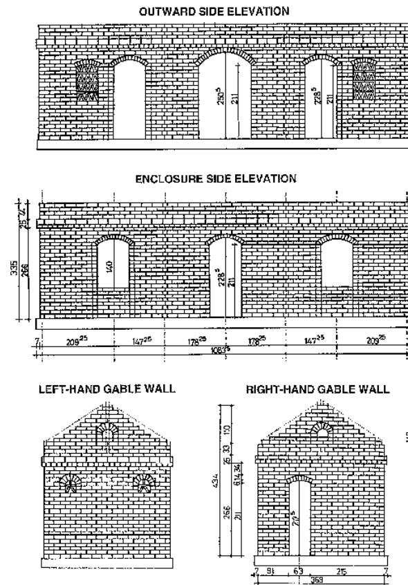
Fig. 219: Detailed coursing of the various elevations of the T3 type housing block.
