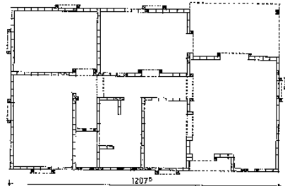
COURSING OF THE SECOND COURSE OF BLOCKS
