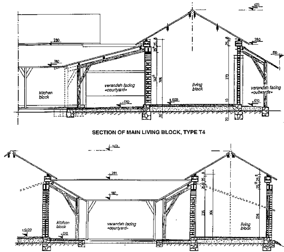
Fig. 215: Sections of type T3 and T4 houses, with verandahs facing "outwards" and towards the "shanza".
