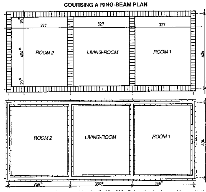
Fig. 222: Above, header course (drawing 11 of fig. 223). Below, the ring-beam sides made of two rows of blocks laid "face on". Note the use of 3/4 blocks at the corners of the building and at the junction of the partition wall with the gutter wall (drawings 111 to V1 of fig. 223).
