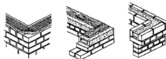
Fig. 120: Ring-beams and reinforced comers using wood or steel embedded in the wall.
