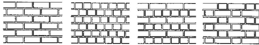
Fig. 45: Fundamental rules of bonding patterns to avoid superimposed vertical joints. (A;B;C;D)
