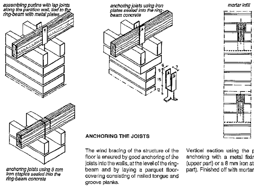
Fig. 272: Detail of systems for anchoring joists into the wall masonry.
