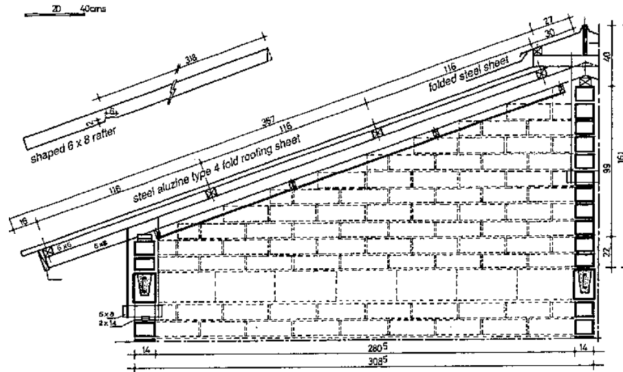
Fig. 141: Ruralhouse, Afatobo, Ivory Coast. Design by CRAterre, S. Maimi. A double sloping roof of steel heets rests on a roof-structure of rafters. These are attached to the masonry of the gutter walls, at the lower side, under a ring-beam made of special sand-cement blocks used as lost formwork, by a stainless steel tie-beam linked to the roof rafter and on one section of rafter passing through the masonry, under the ring-beam. At the top, a ridge ventilator is itself fixed to the partition wan using the same principle.
