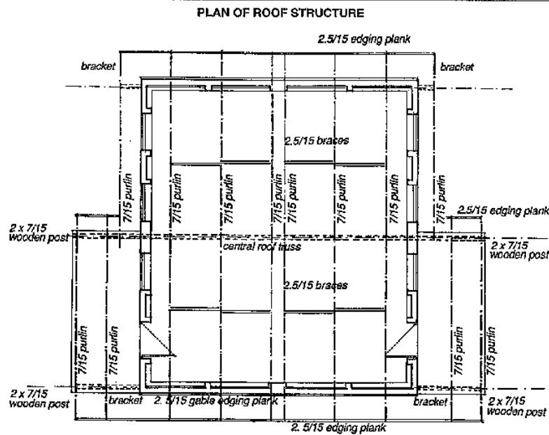
Fig. 312: Plan of roof structure detailing the wood sections and the principle of horizontal wind-bracina by bridging the purlins.
