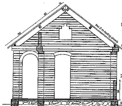
Fig. 196: Section AA figs. 192 and 193. Note the arches: semi-circular (verandah), Dutch (doors and windows), and corbel (upper ventilation of the gable-end).
