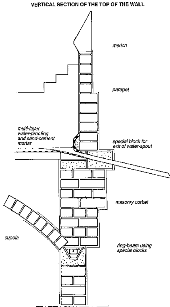
Fig. 332: Vertical section of the external wall from the ring-beam to the merlon.
