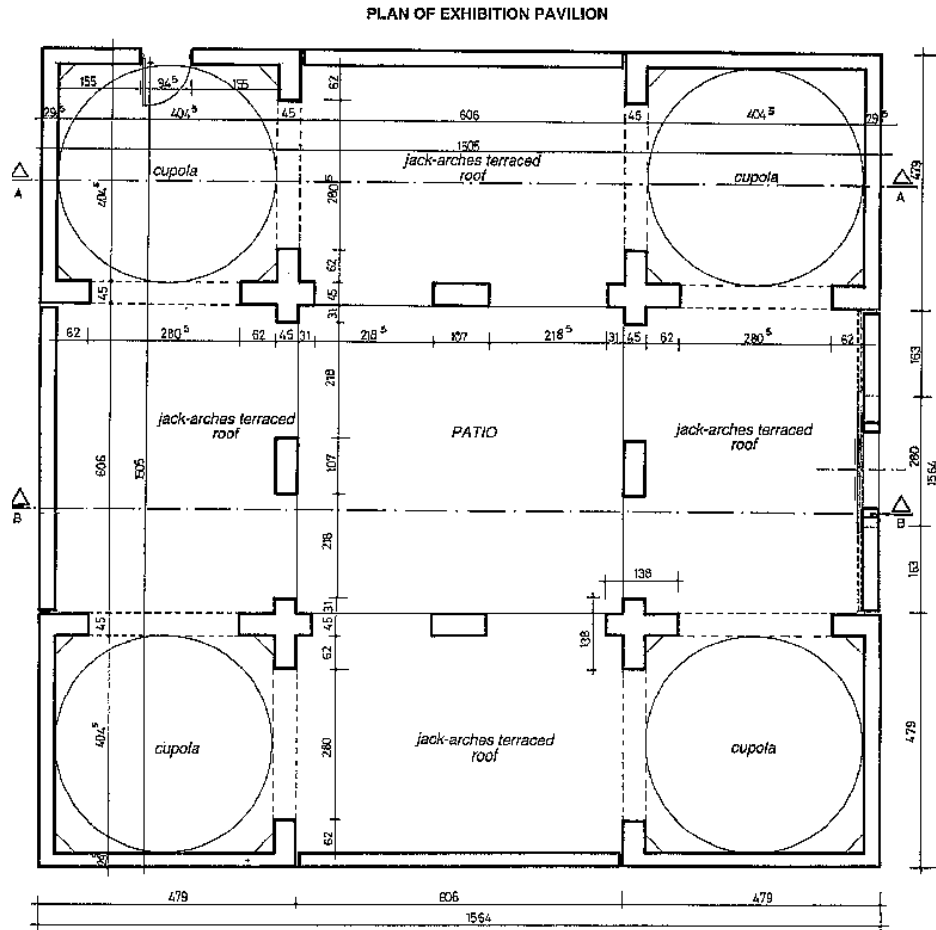
Fig. 319: Plan of square exhibition pavilion, with cupolas at each of the four corners connected by vaulted spaces around an interior courtyard.
