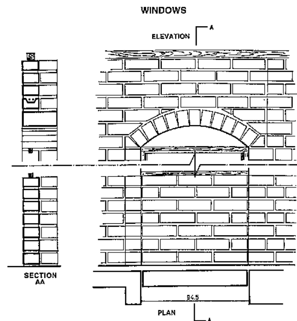
Fig. 315: Plan, elevation and vertical section of a «naco» frame window opening.
