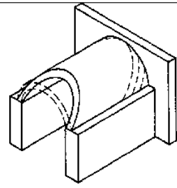
"Nubian" vault with inclined courses
