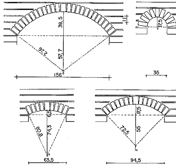
Fig. 220: Types of Dutch and semi-circular arches used in the project.
