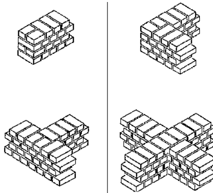
Fig. 57: A few examples of header bonding patterns for walls one block thick.
